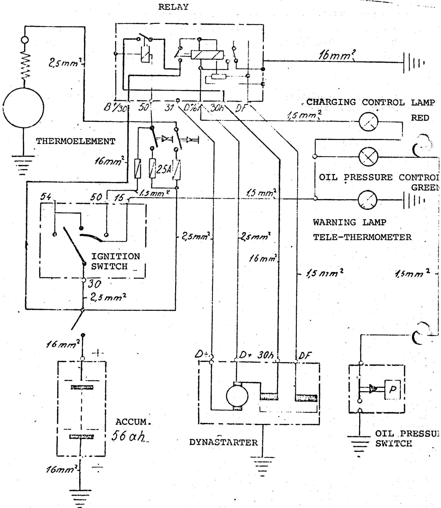
Wiring diagram for dynastarter with thermostart and instrument panel.
